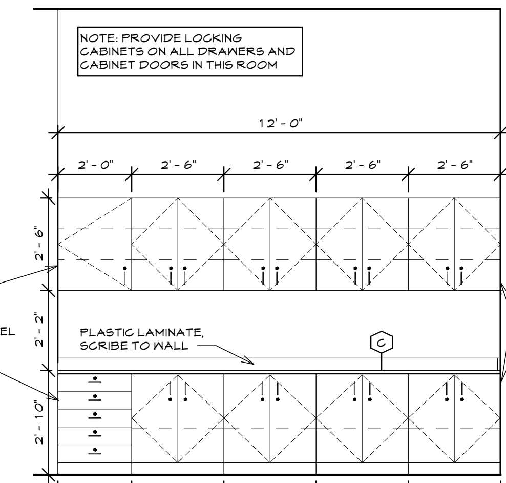
⑯ SERVING LINE SCALE: 3/8" = 1'-0" ROOM 216
