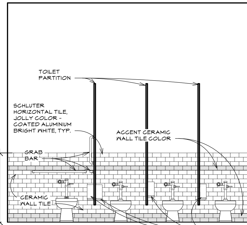
⑥ WOMEN'S R.R. SCALE: 3/8" = 1'-0" ROOM 206
