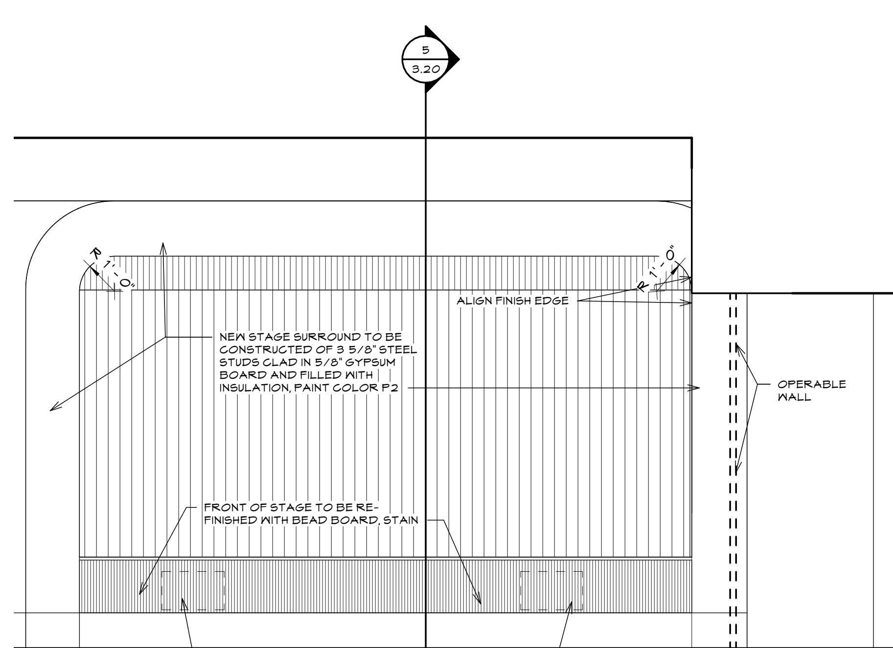
㉕ STAGE SCALE: 3/8" = 1'-0" ROOM 212
