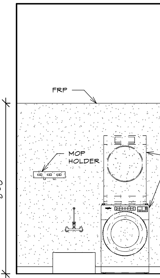
⑨ JANITOR'S CLST. SCALE: 3/8" = 1'-0" ROOM 221
