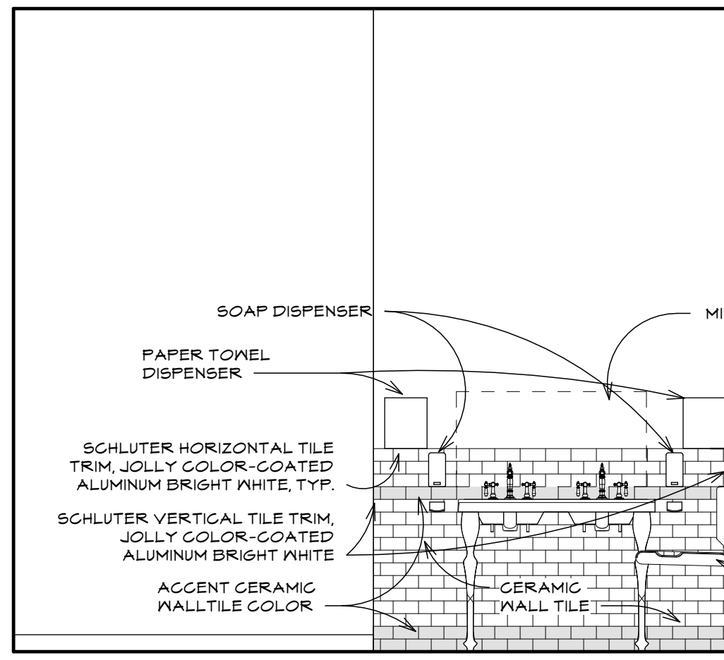
③ MEN'S R.R. SCALE: 3/8" = 1'-0" ROOM 204
