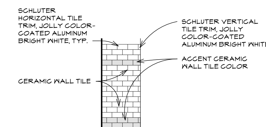
⑭ HALL SCALE: 3/8" = 1'-0" ROOM 205
