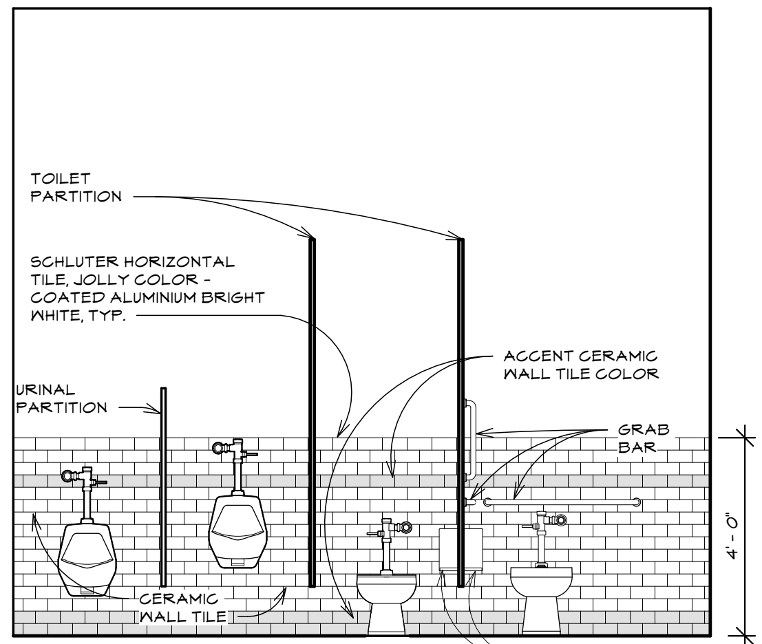
① MEN'S R.R. SCALE: 3/8" = 1'-0" ROOM 204
