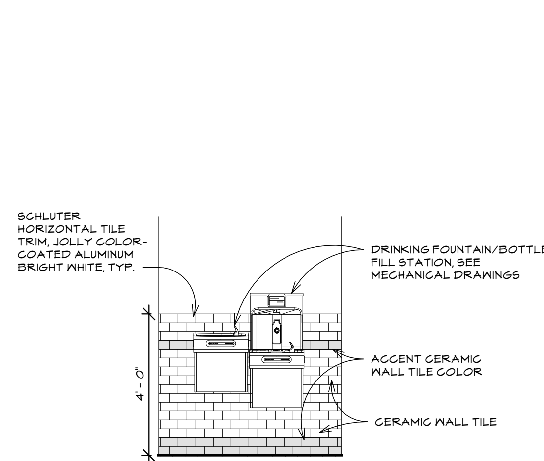
⑪ HALL SCALE: 3/8" = 1'-0" ROOM 205
