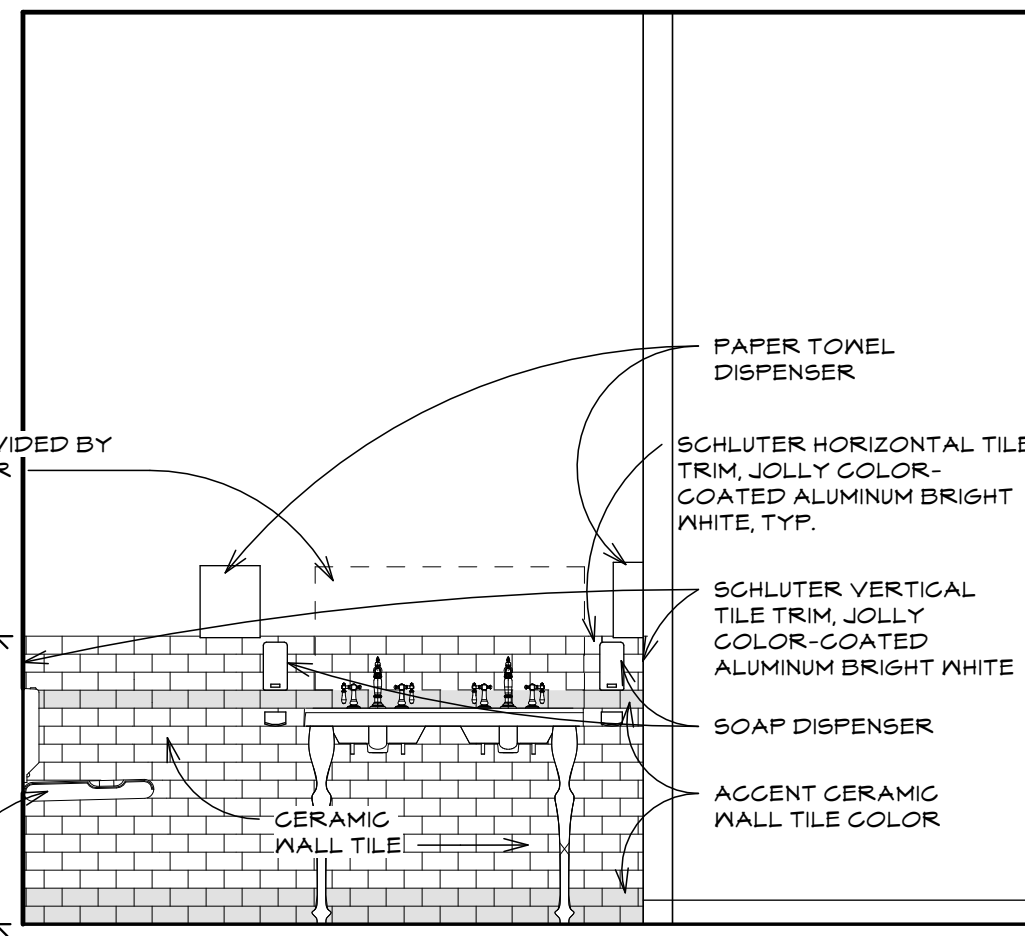
④ WOMEN'S R.R. SCALE: 3/8" = 1'-0" ROOM 206
