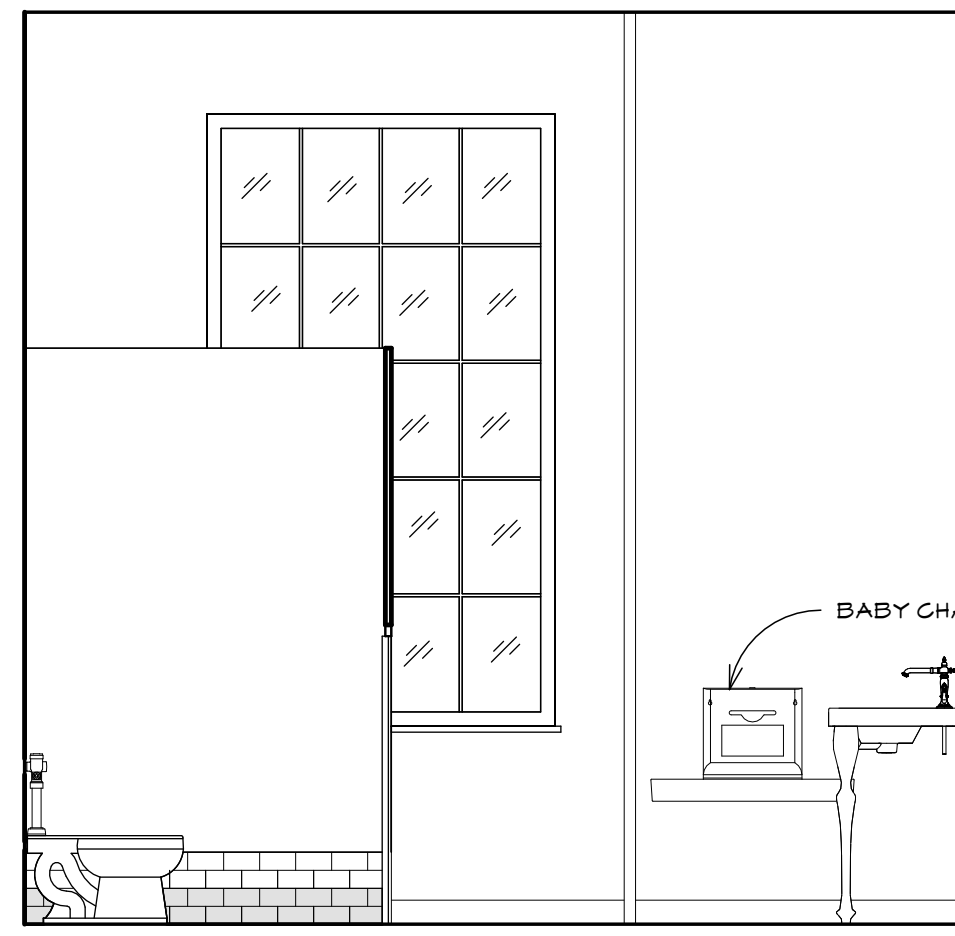
⑤ WOMEN'S R.R. SCALE: 3/8" = 1'-0" ROOM 206
