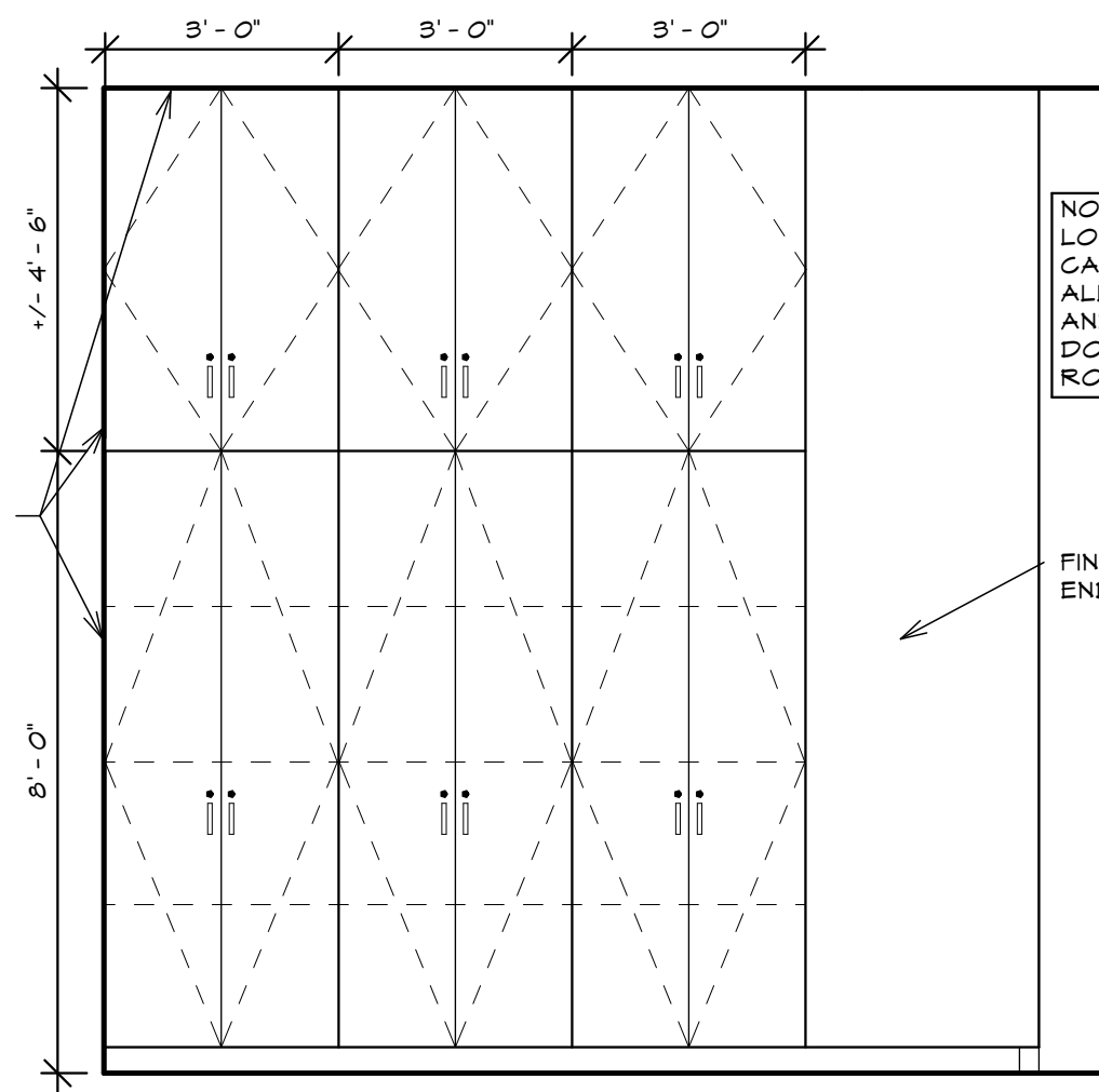
⑱ LOBBY SCALE: 3/8" = 1'-0" ROOM 216
