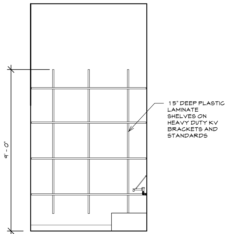
⑩ JANITOR'S CLST. SCALE: 3/8" = 1'-0" ROOM 221
